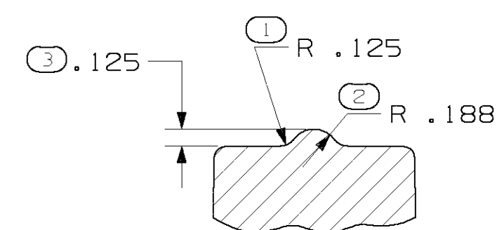
SECTION A-A (B5)
