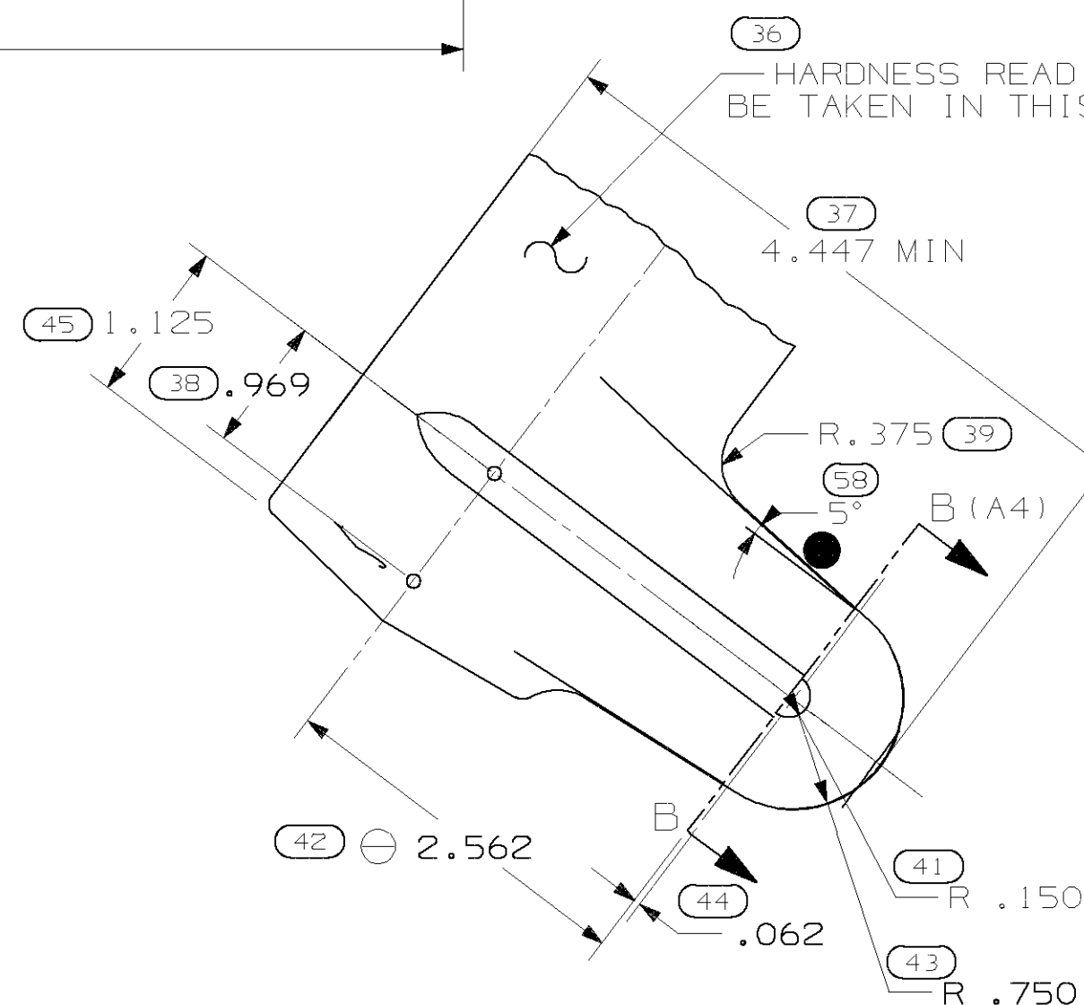
VIEW AT "C" (A7)
