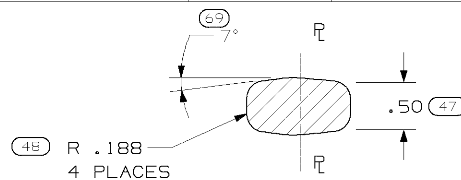
SECTION B-B (D5)
